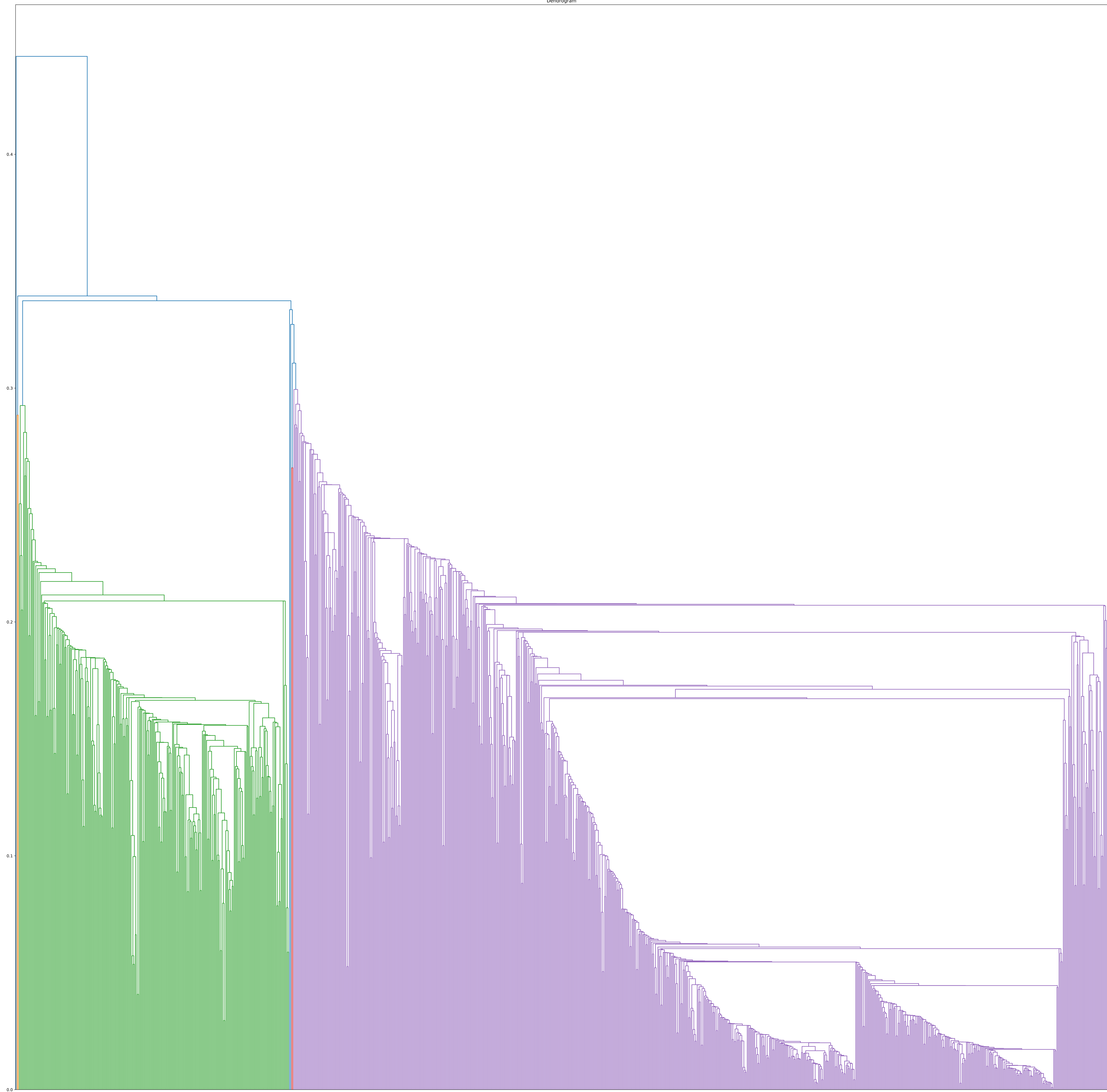
Dendrogram
