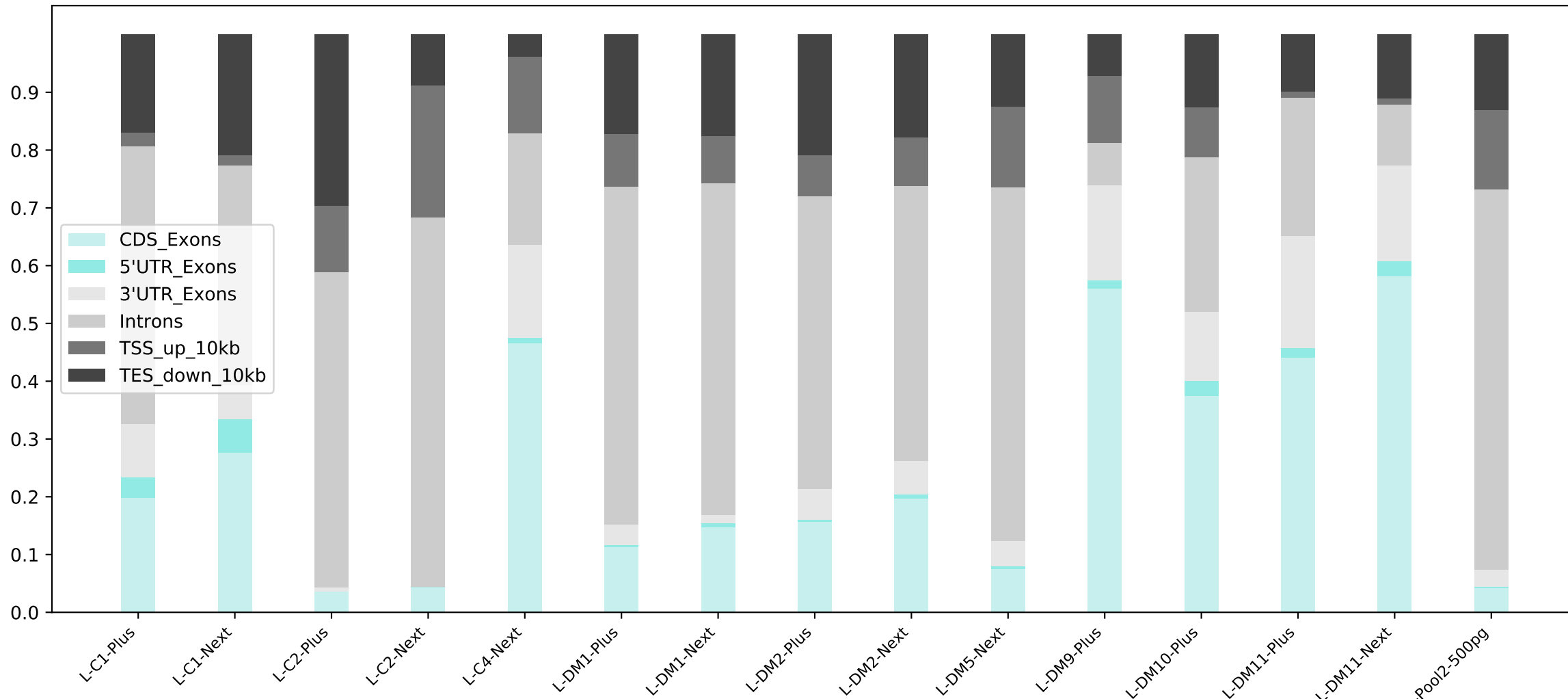
Read Distribution
