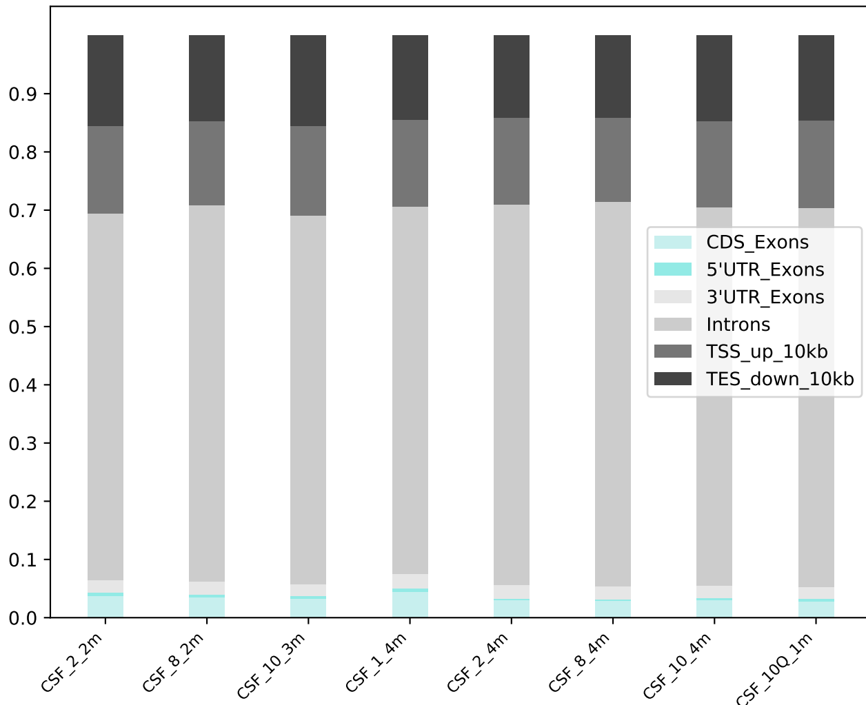
Read Distribution
