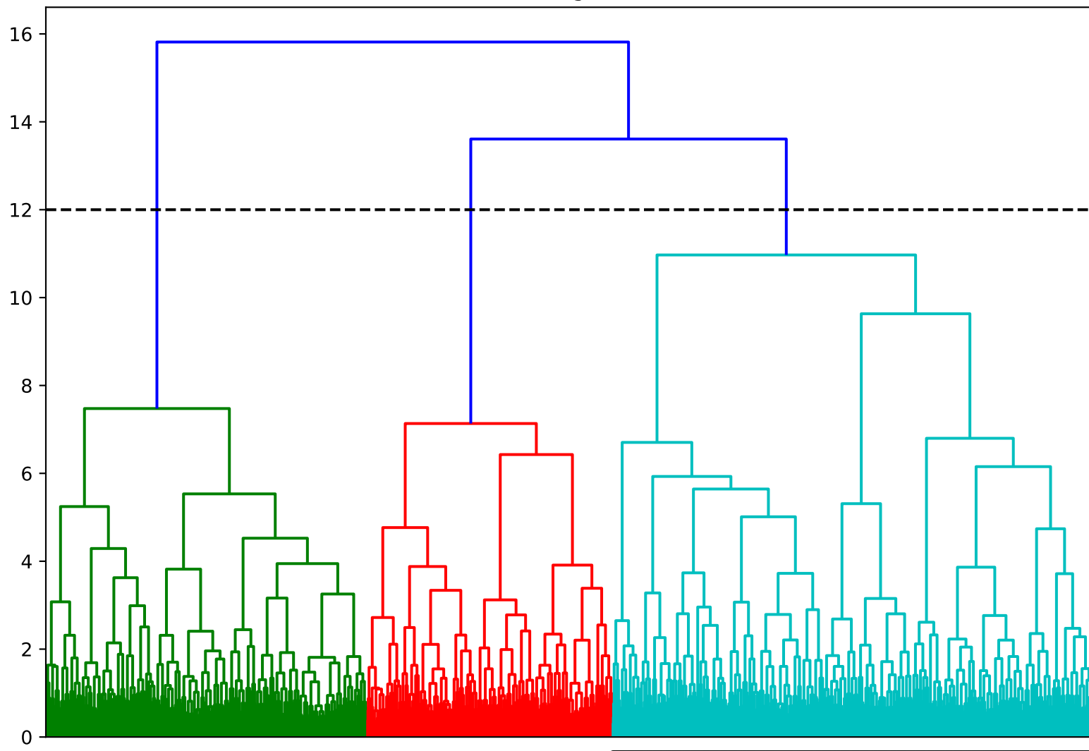
Dendrograms
