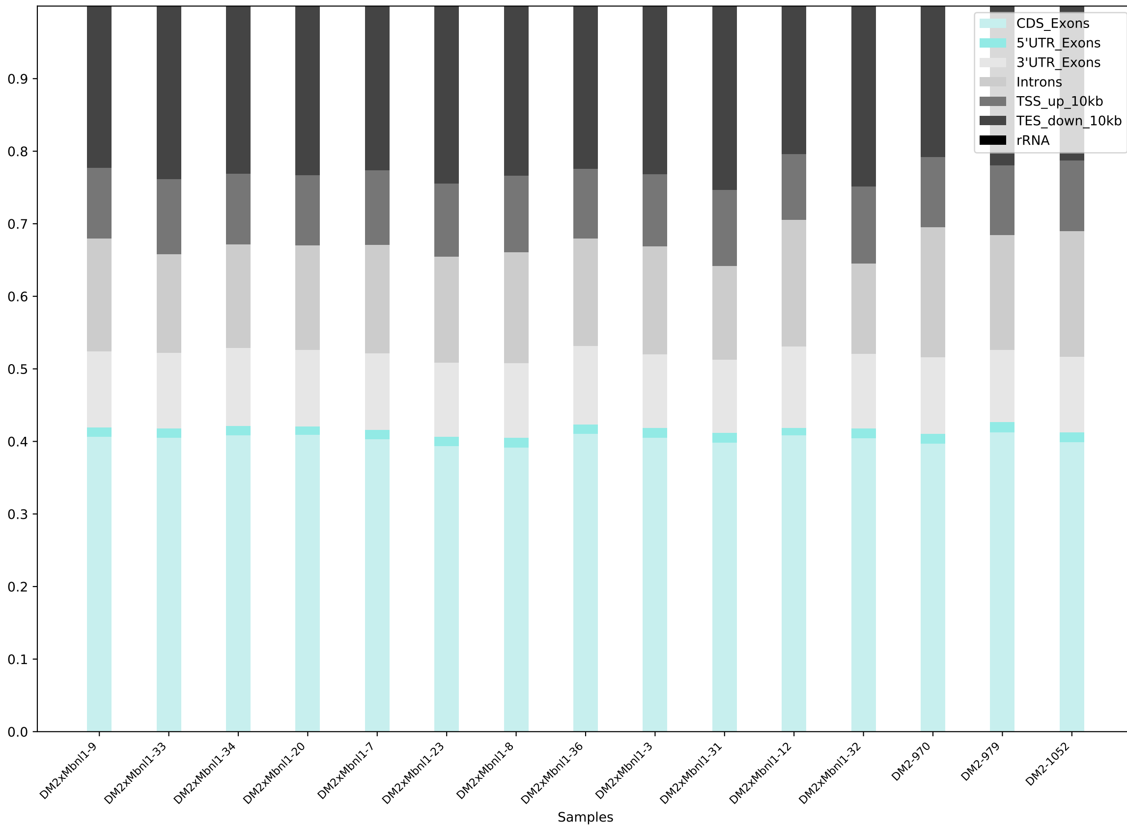
Read Distribution
