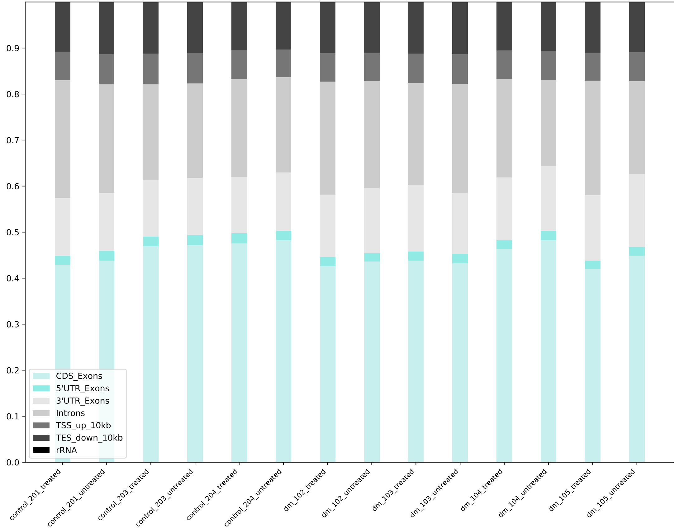
Read Distribution
