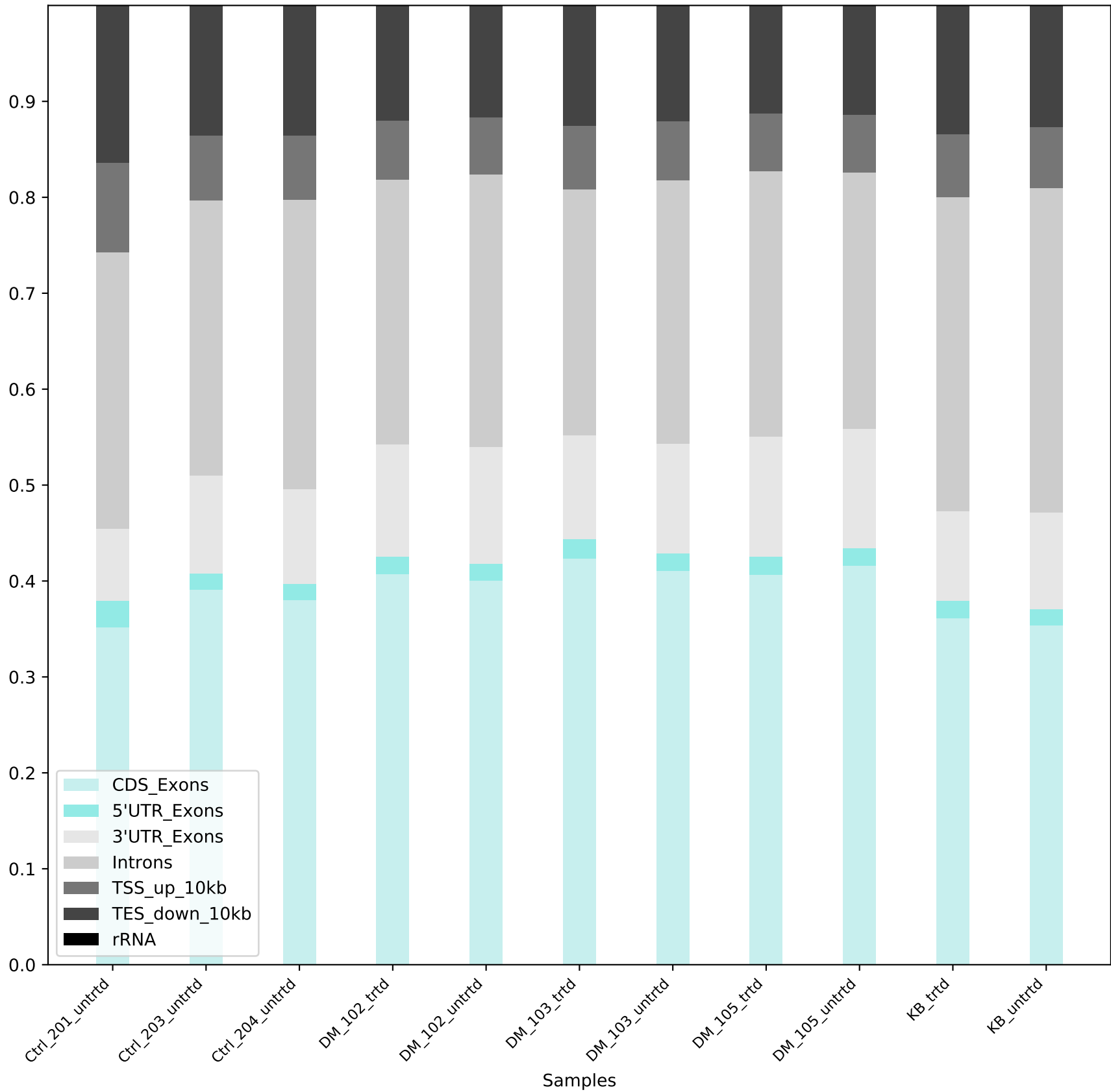
Read Distribution
