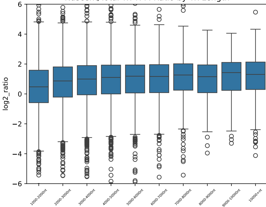
Nascent/Total Tx TPM Ratio by Tx Length
