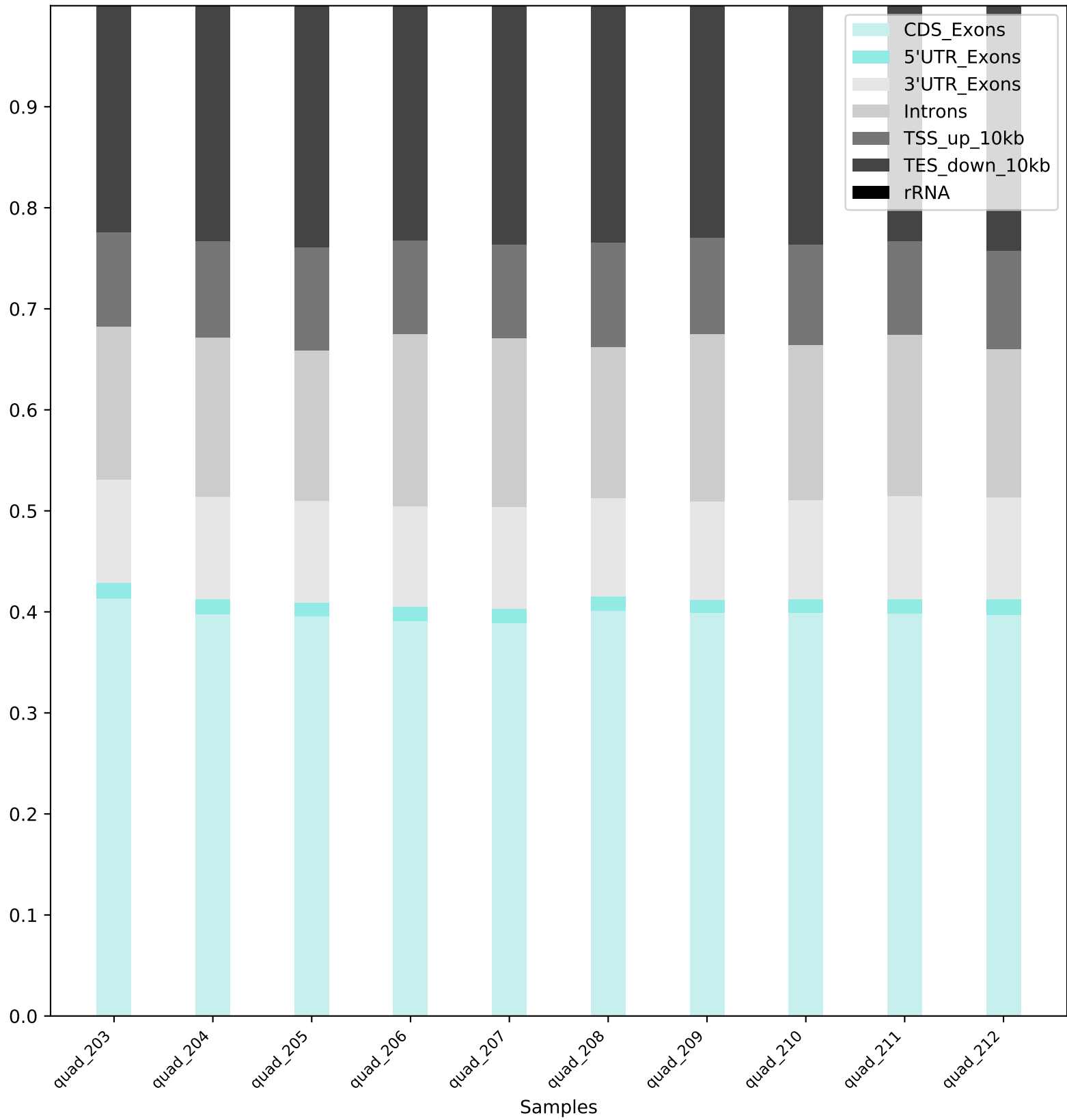
Read Distribution
